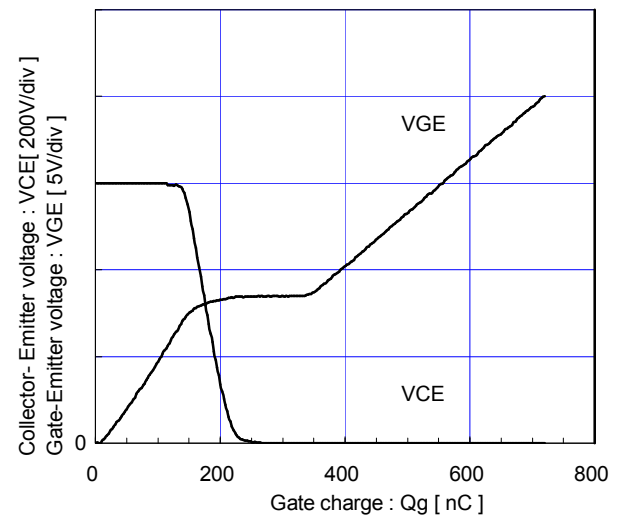
Dynamic Gate charge (typ.) Vcc=600V, Ic=150A, Tj=25°C
