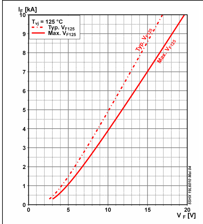
Fig. 10 Max. on-state voltage characteristics
