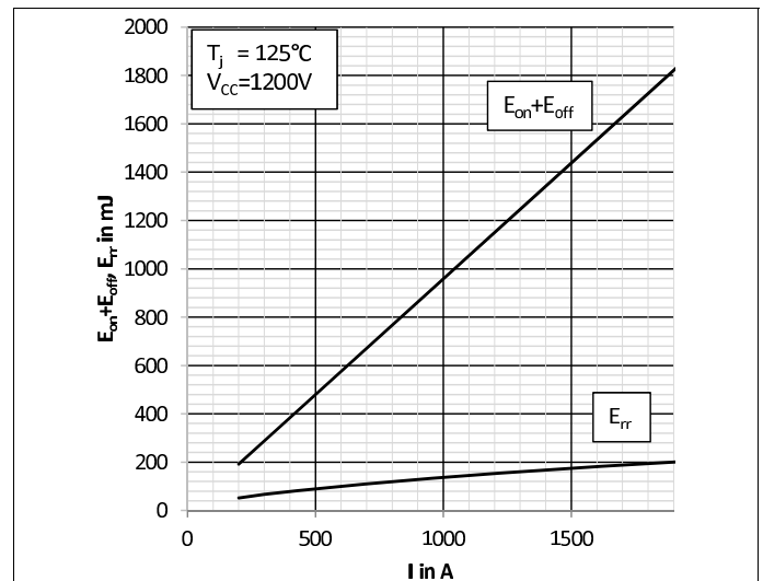
Fig. 4: Typical energy losses E = f(I_C, V_{CE})
