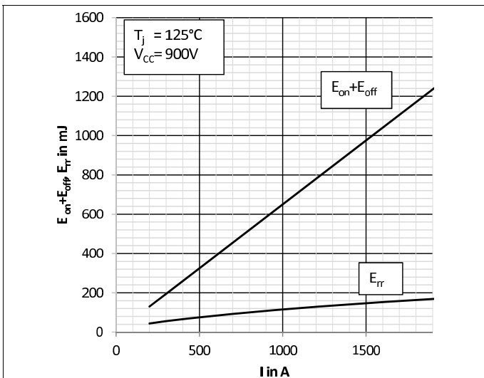
Fig. 3: Typical energy losses E = f(I_C, V_{CE})
