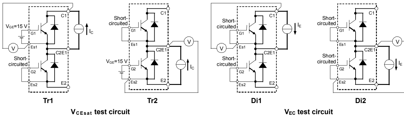
Tr1/Tr2: IGBT, Di1/Di2: FWDi
