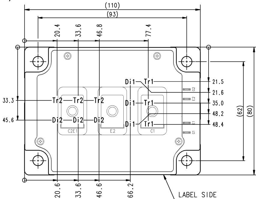
Tr1/Tr2: IGBT, Di1/Di2: FWDi
