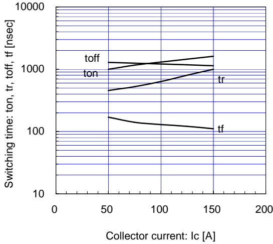
Switching time vs. Collector current (typ.) V_{cc}=900V, V_{GE}=\pm 15V, R_g=22\Omega, T_j=125^\circ C
