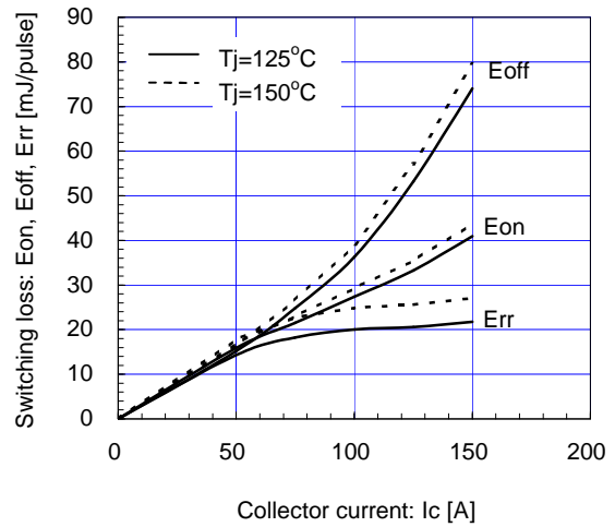
Switching loss vs. Collector current (typ.) V_{cc}=900, V_{GE}=\pm 15V, R_g=22\Omega, T_j=125, 150^\circ C
