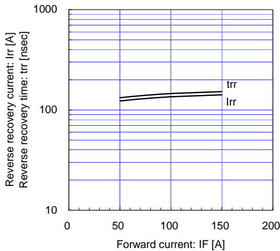
Reverse Recovery Characteristics (typ.) Vcc=900V, VGE=±15V, Rg=22Ω, Tj=150°C
