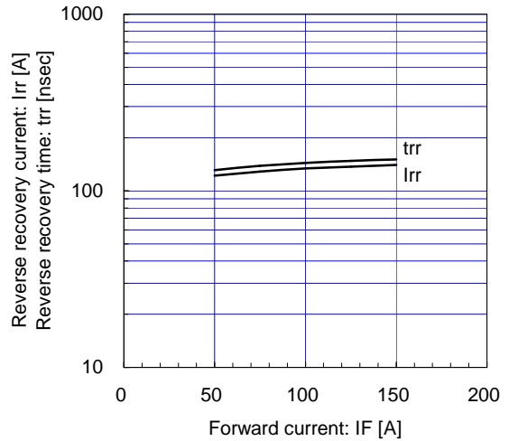
Reverse Recovery Characteristics (typ.) Vcc=900V, VGE=±15V, Rg=22Ω, Tj=125°C
