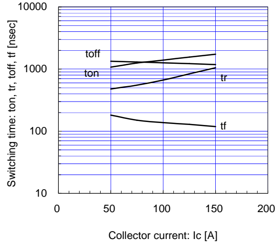
Switching time vs. Collector current (typ.) V_{cc}=900V, V_{GE}=\pm 15V, R_g=22\Omega, T_j=150^\circ C
