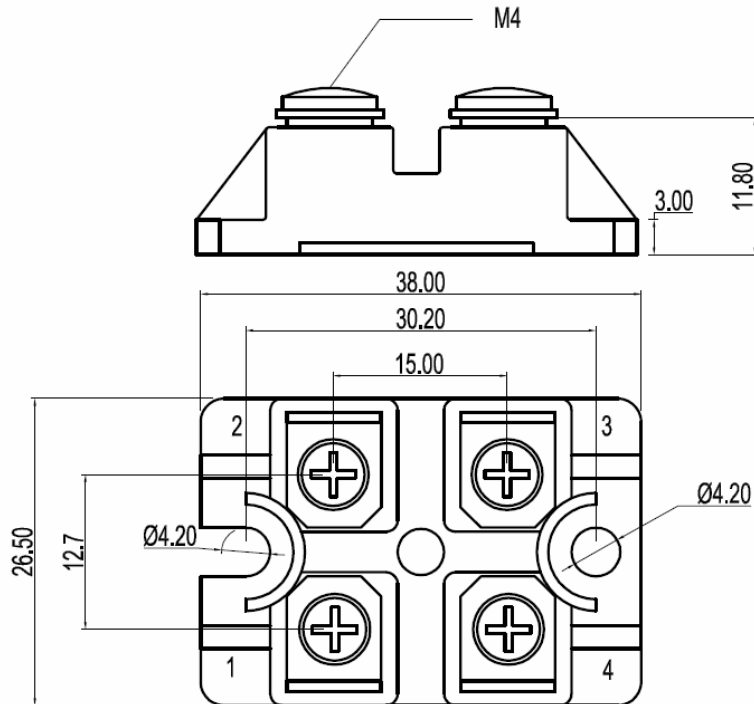
Dimensions (mm) Figure7. Package Outline
