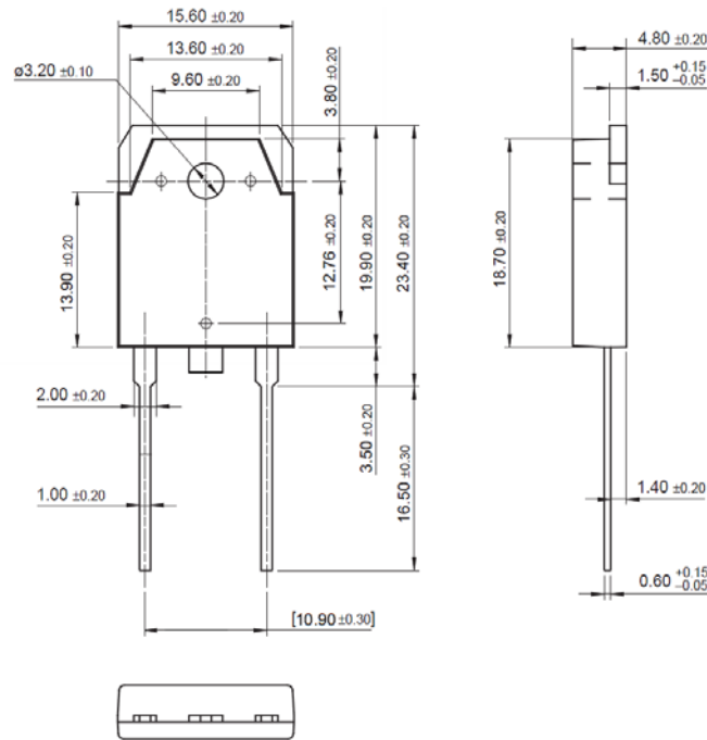
Fig8. Package Outline
