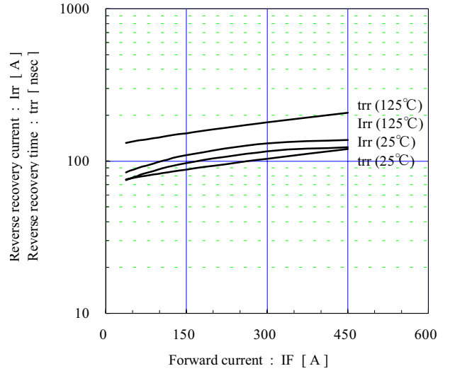
Reverse recovery characteristics (typ.) V_{cc}=300V, V_{GE}=\pm 15V, R_g=9.1\Omega
